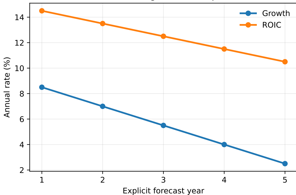
Linear convergence assumptions
